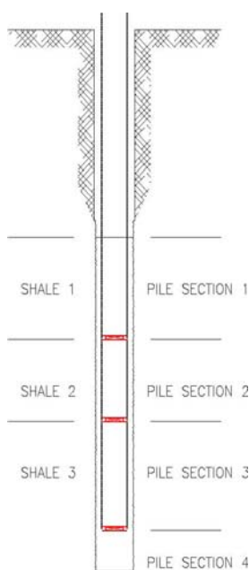
Schematic elevation of test pile showing position of three levels of O-cells and deep concrete cut-off
