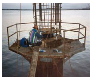
Installation of Pile Cage with O-cell assembly attached
