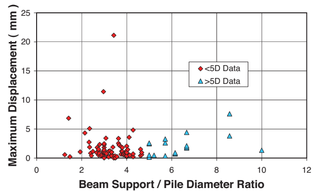
[FIG. 3] Maximum Reference Beam Displacement vs. Support/Pile Diameter Ratio (LOADTEST Database, 1995-2004)
