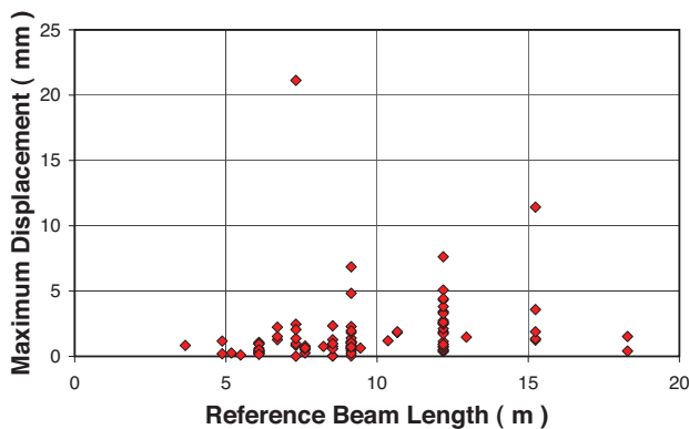
[FIG. 2] Maximum Reference Beam Displacement vs. Beam Length (LOADTEST Database, 1995-2004)
