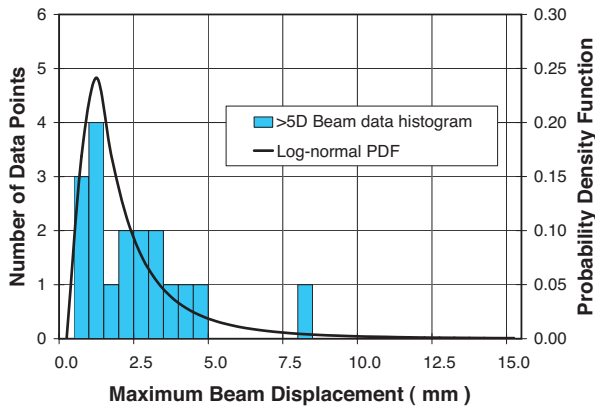
[FIG. 5] Probability Density Function (PDF) of Max. Beam Displacement (>5D Subset) (LOADTEST Database, 1995-2004)
