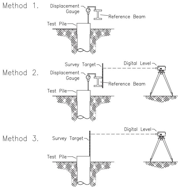
[FIG. 1] Schematics of Pile Head Displacement Measurement Methods
