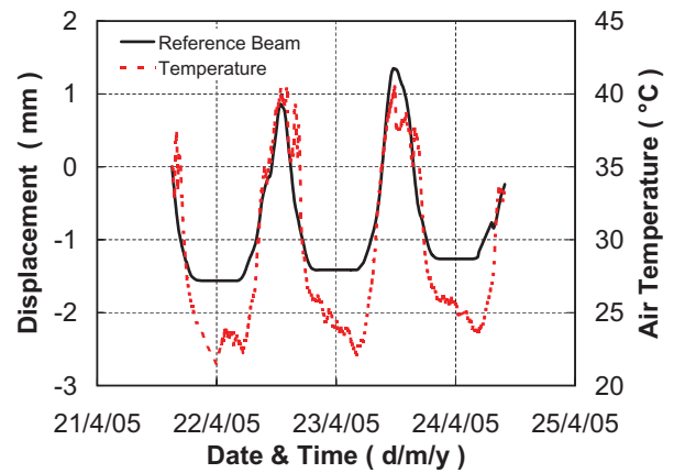
[FIG. 7] Shaded Reference Beam Displacement Compared with Temperature Variation (LOADTEST Project Reference No. 213-3, 2005)
