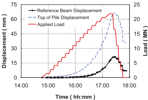
[FIG. 6] Reference Beam Displacement Compared with Applied Load (LOADTEST Project Reference No. 620, 2004)
