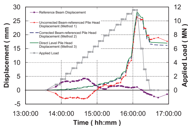
[FIG. 8] Direct Comparison of Results of Method 2 and Method 3 (LOADTEST Project Reference No. 539, 2005)
