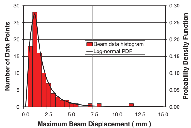
[FIG. 4] Probability Density Function (PDF) of Max. Beam Displacement (LOADTEST Database, 1995-2004)
