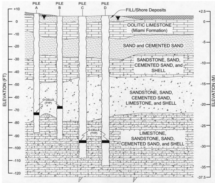
Figure 2 – Geological Profile
