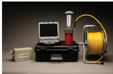
The SONICaliper equipment
